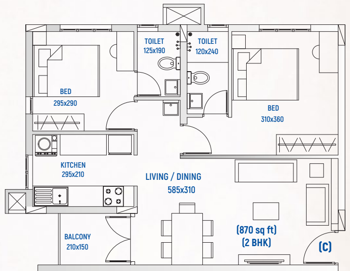
C - TYPE (2 BHK) AREA - 870 sq ft
