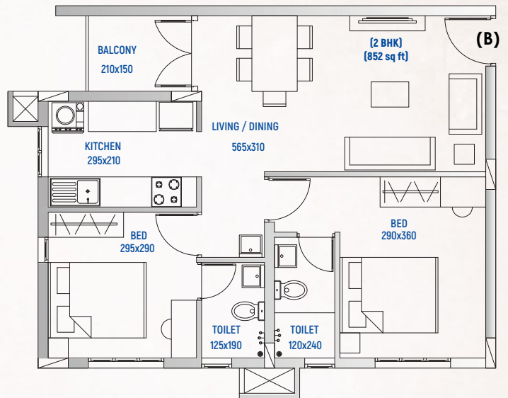
B - TYPE (2 BHK) AREA - 852 sq ft
