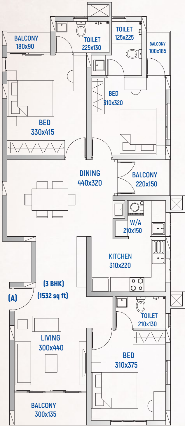
A - TYPE (3 BHK) AREA - 1532 sq ft
